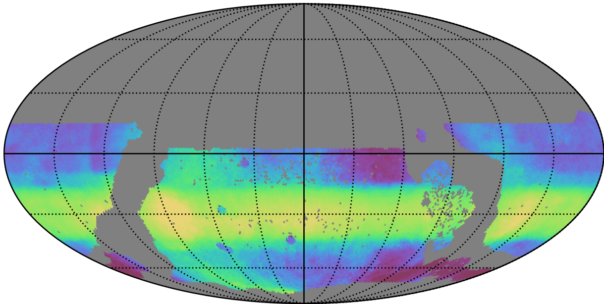
too_elab_r32_d3_griz_v3.4_10yrs WFD all bands: Median HA
