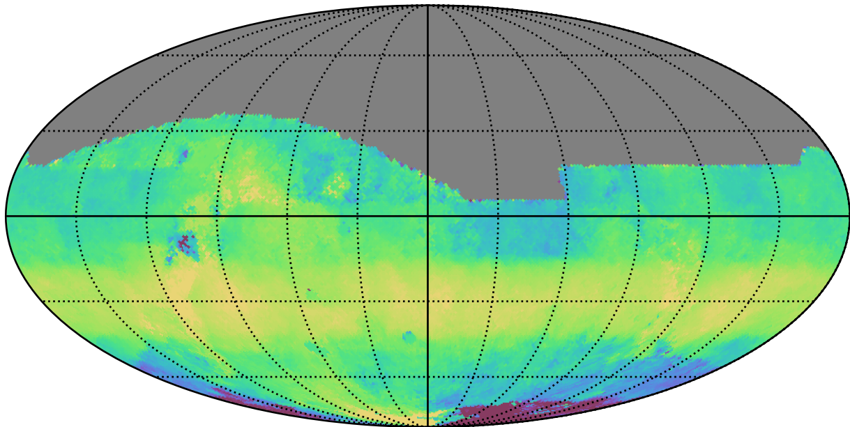
too_elab_r32_d3_griz_v3.4_10yrs All sky z band: Median HA
