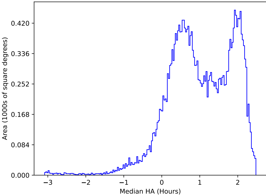
too_elab_r32_d3_griz_v3.4_10yrs All sky z band: Median HA
