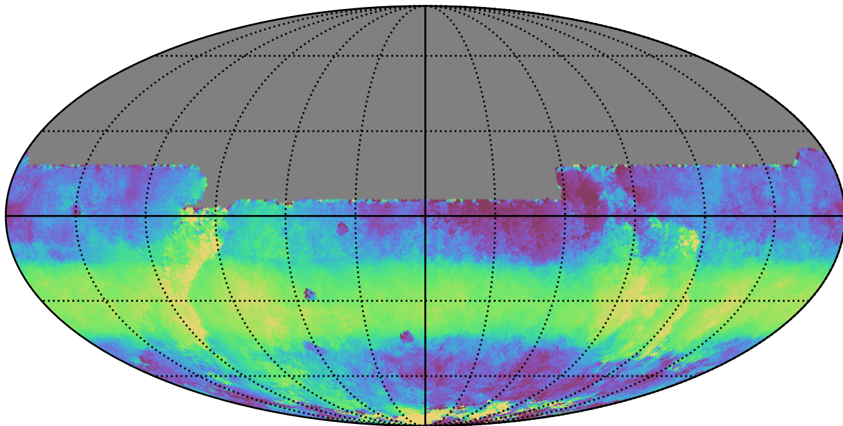
too_elab_r32_d3_griz_v3.4_10yrs All sky y band: Median HA
