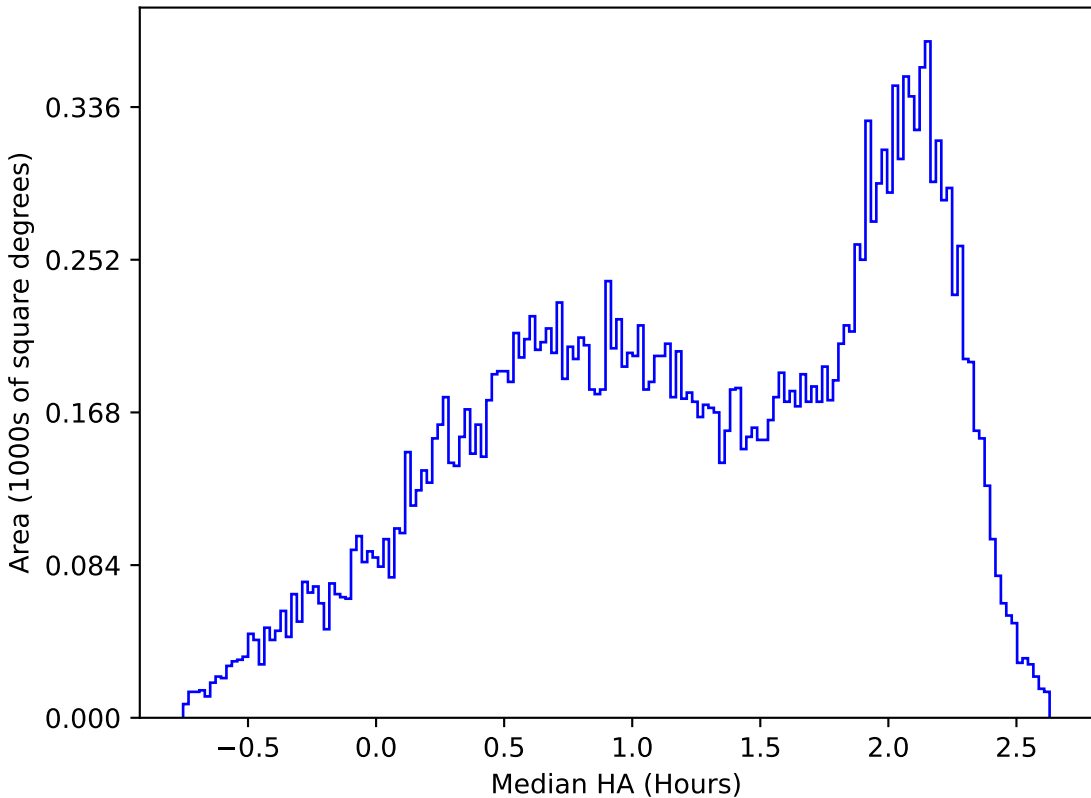
too_elab_r32_d3_griz_v3.4_10yrs All sky y band: Median HA
