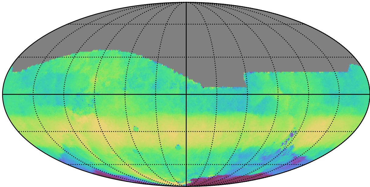
too_elab_r32_d3_griz_v3.4_10yrs All sky r band: Median HA
