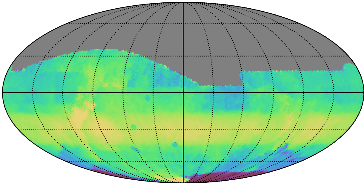
too_elab_r32_d3_griz_v3.4_10yrs All sky i band: Median HA
