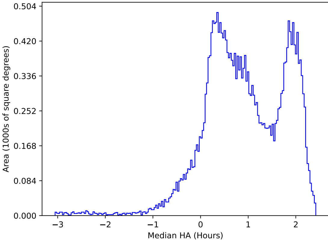
too_elab_r32_d3_griz_v3.4_10yrs All sky i band: Median HA
