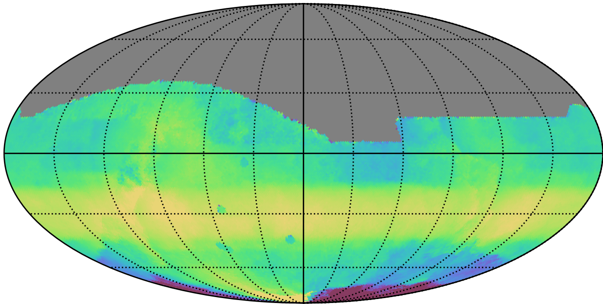
too_elab_r32_d3_griz_v3.4_10yrs All sky all bands: Median HA
