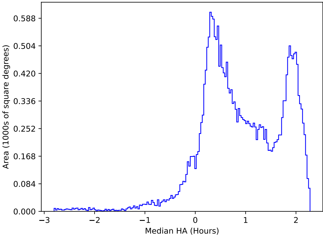
too_elab_r32_d3_griz_v3.4_10yrs All sky all bands: Median HA
