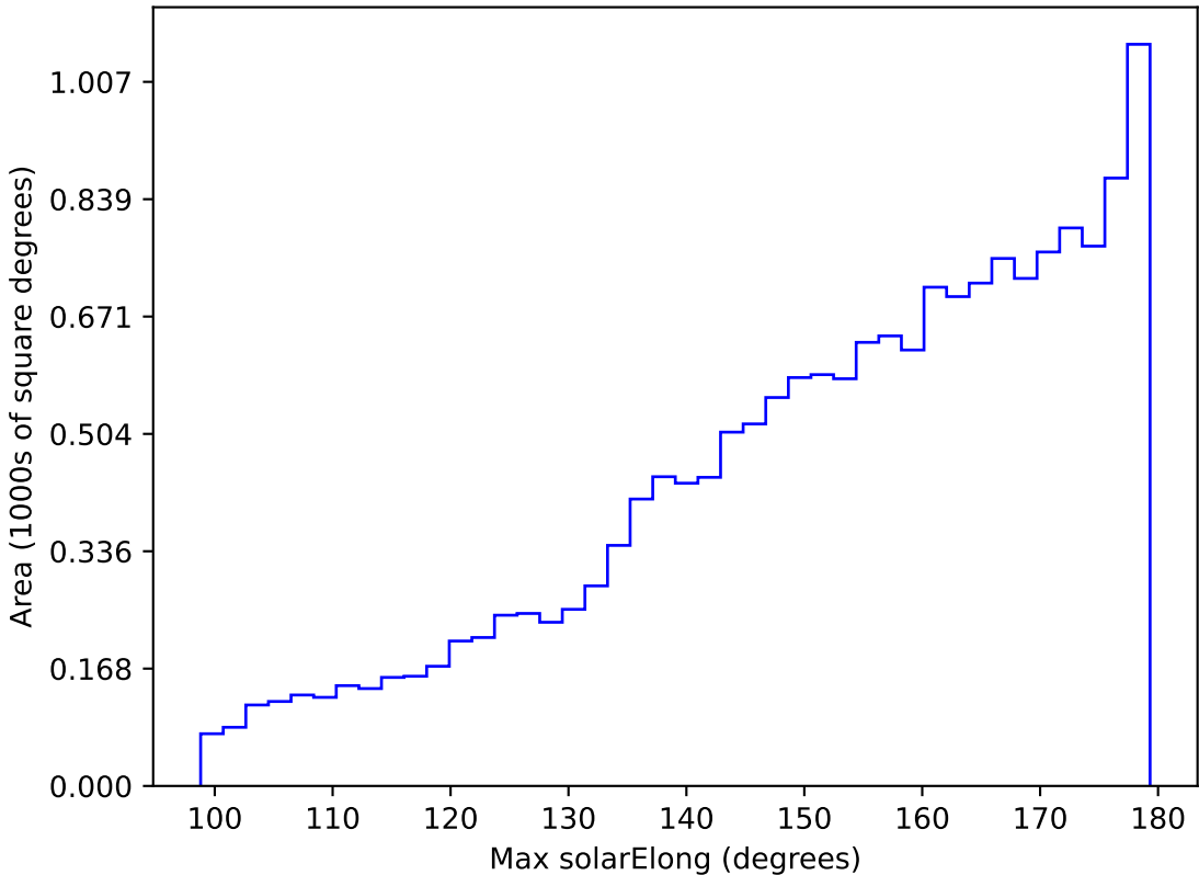
too_elab_r32_d3_griz_v3.4_10yrs WFD z band: Max solarElong
