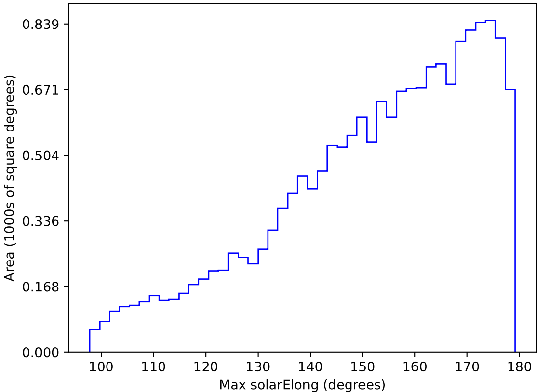
too_elab_r32_d3_griz_v3.4_10yrs WFD u band: Max solarElong
