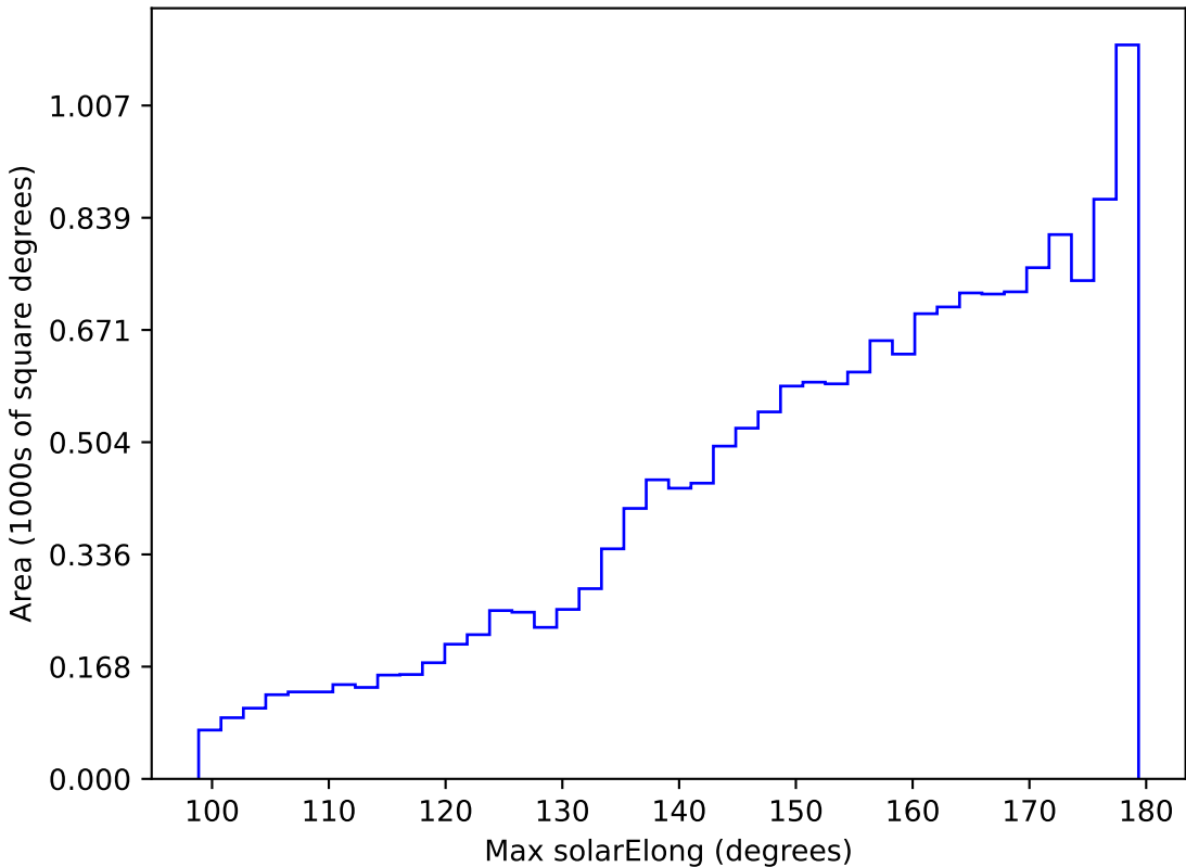
too_elab_r32_d3_griz_v3.4_10yrs WFD i band: Max solarElong
