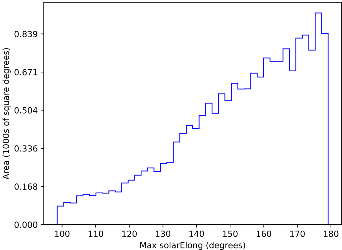
too_elab_r32_d3_griz_v3.4_10yrs WFD g band: Max solarElong
