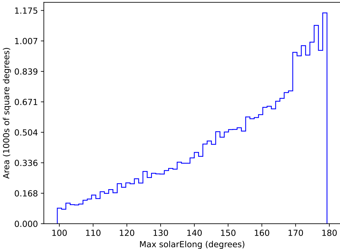
too_elab_r32_d3_griz_v3.4_10yrs All sky z band: Max solarElong
