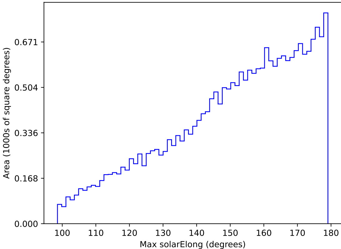
too_elab_r32_d3_griz_v3.4_10yrs All sky y band: Max solarElong
