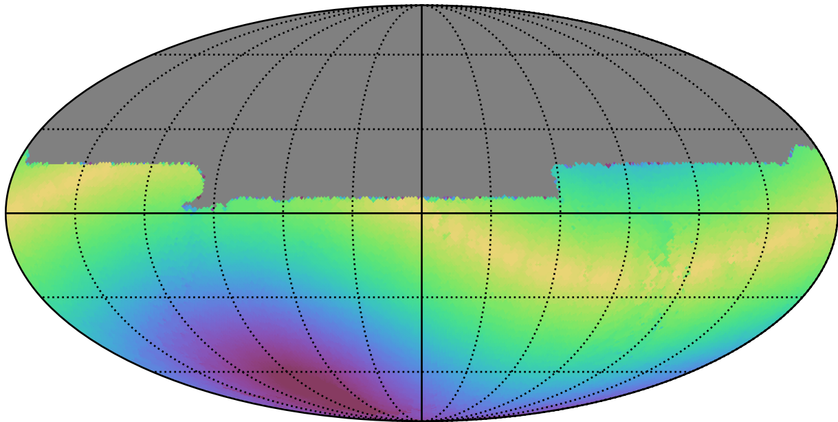
too_elab_r32_d3_griz_v3.4_10yrs All sky u band: Max solarElong
