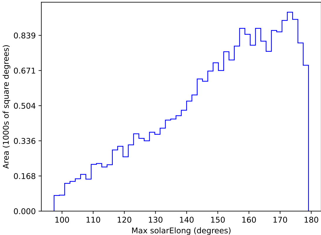
too_elab_r32_d3_griz_v3.4_10yrs All sky u band: Max solarElong
