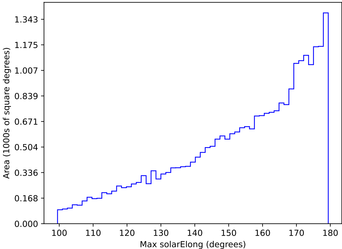
too_elab_r32_d3_griz_v3.4_10yrs All sky r band: Max solarElong
