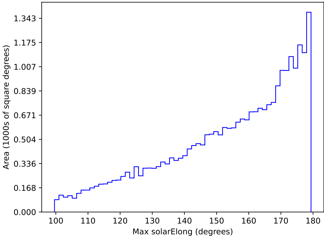
too_elab_r32_d3_griz_v3.4_10yrs All sky i band: Max solarElong
