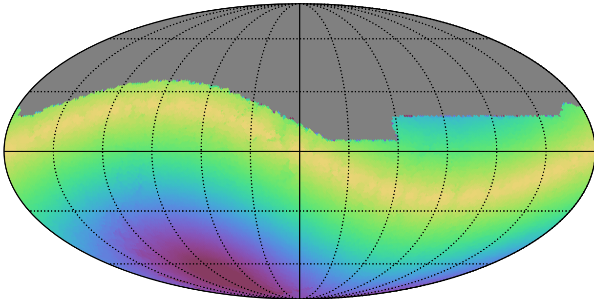
too_elab_r32_d3_griz_v3.4_10yrs All sky g band: Max solarElong
