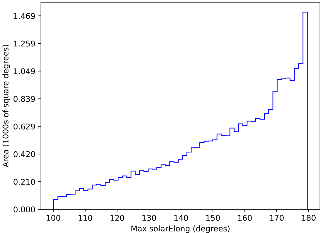
too_elab_r32_d3_griz_v3.4_10yrs All sky all bands: Max solarElong
