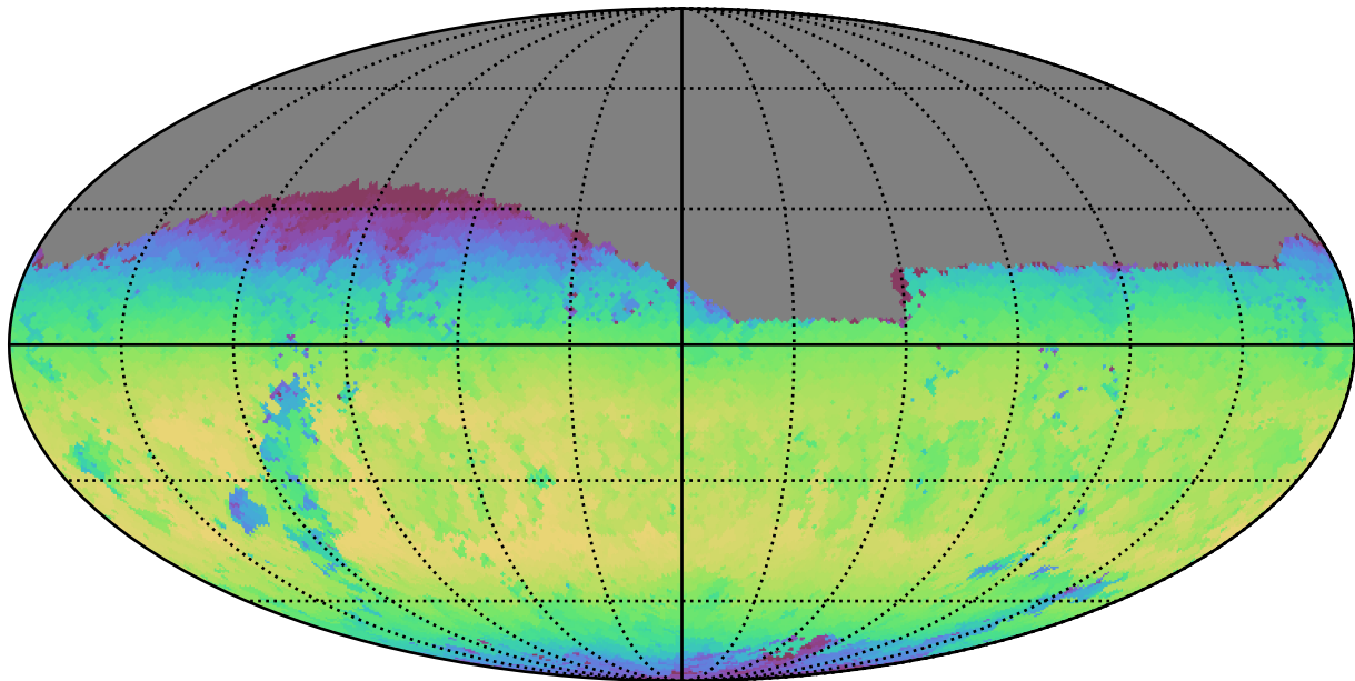
too_elab_r32_d3_griz_v3.4_10yrs Yr 1 z band: Max skyBrightness
