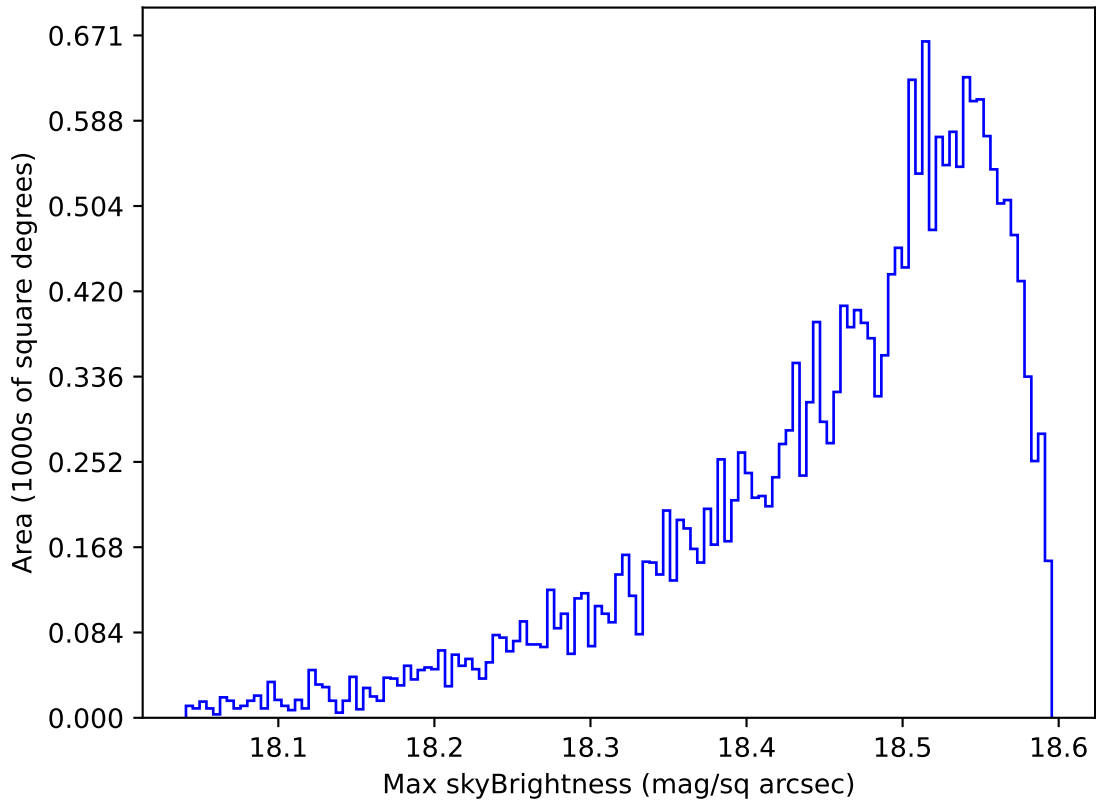
too_elab_r32_d3_griz_v3.4_10yrs Yr 1 y band: Max skyBrightness
