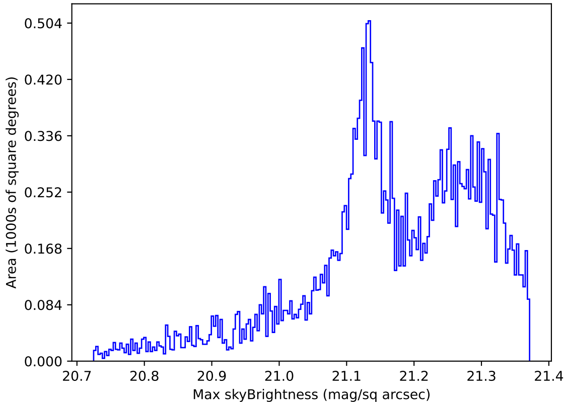
too_elab_r32_d3_griz_v3.4_10yrs Yr 1 r band: Max skyBrightness
