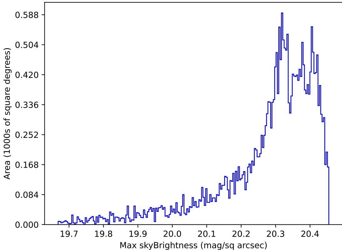
too_elab_r32_d3_griz_v3.4_10yrs Yr 1 i band: Max skyBrightness
