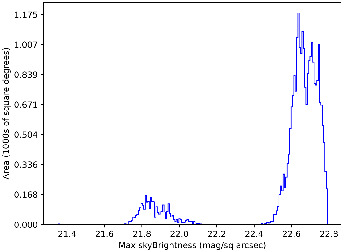
too_elab_r32_d3_griz_v3.4_10yrs Yr 1 all bands: Max skyBrightness
