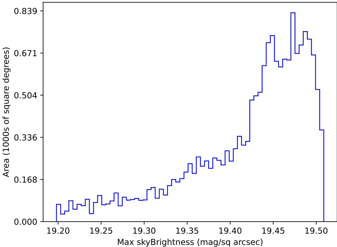
too_elab_r32_d3_griz_v3.4_10yrs WFD z band: Max skyBrightness
