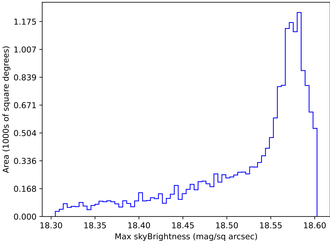
too_elab_r32_d3_griz_v3.4_10yrs WFD y band: Max skyBrightness
