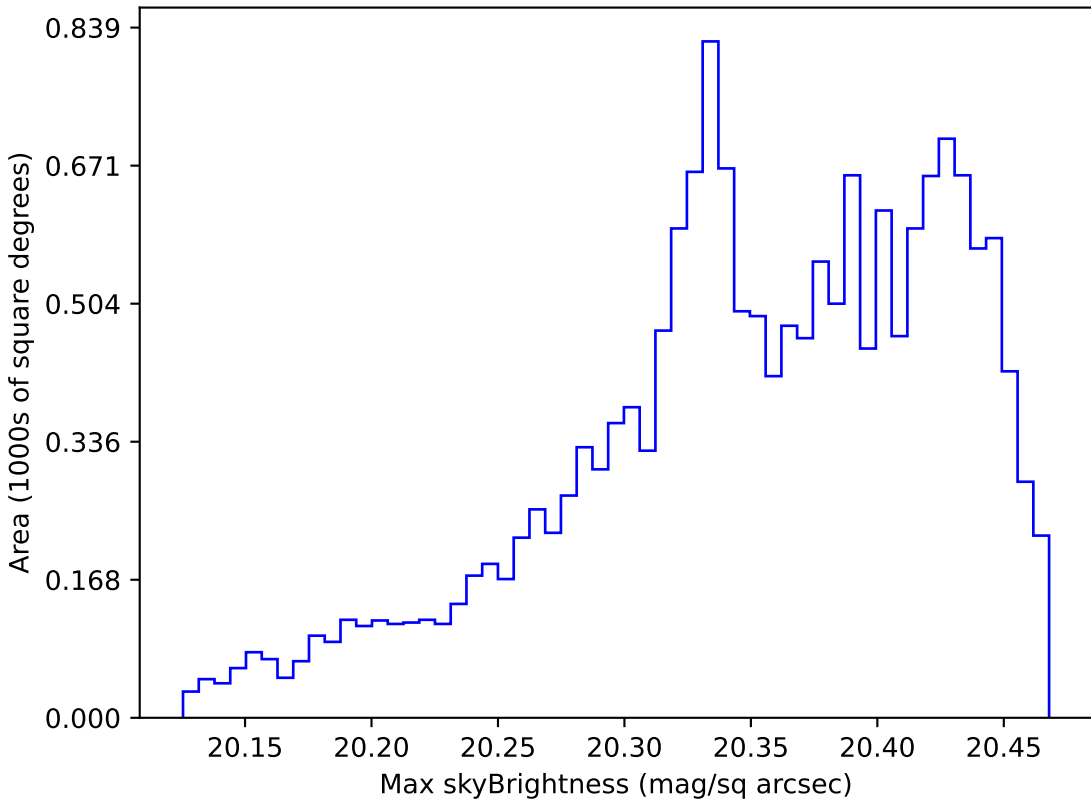
too_elab_r32_d3_griz_v3.4_10yrs WFD i band: Max skyBrightness
