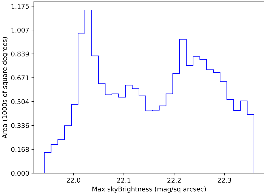
too_elab_r32_d3_griz_v3.4_10yrs WFD g band: Max skyBrightness
