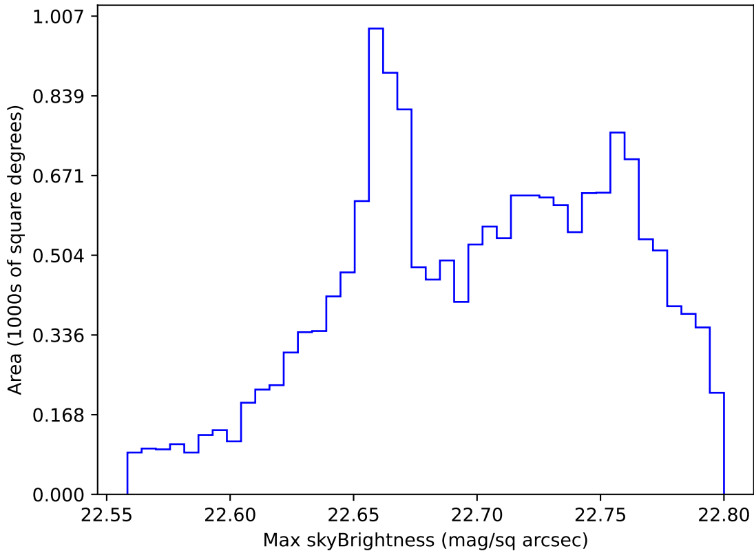
too_elab_r32_d3_griz_v3.4_10yrs WFD all bands: Max skyBrightness
