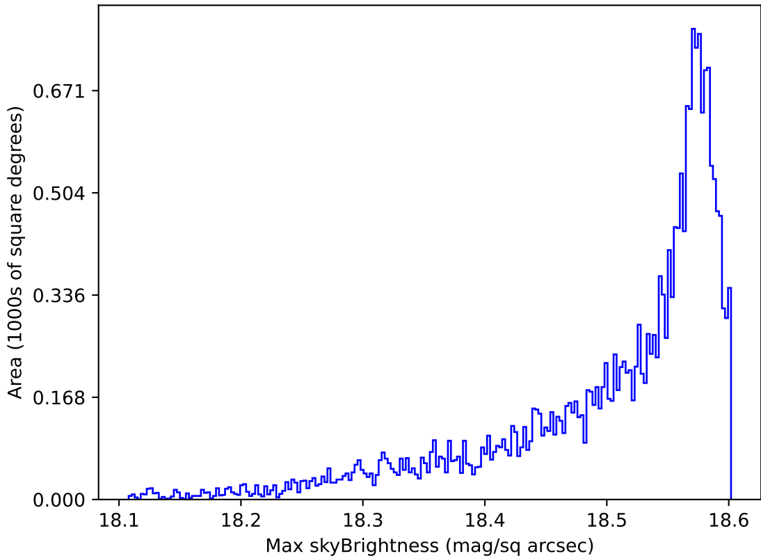
too_elab_r32_d3_griz_v3.4_10yrs All sky y band: Max skyBrightness
