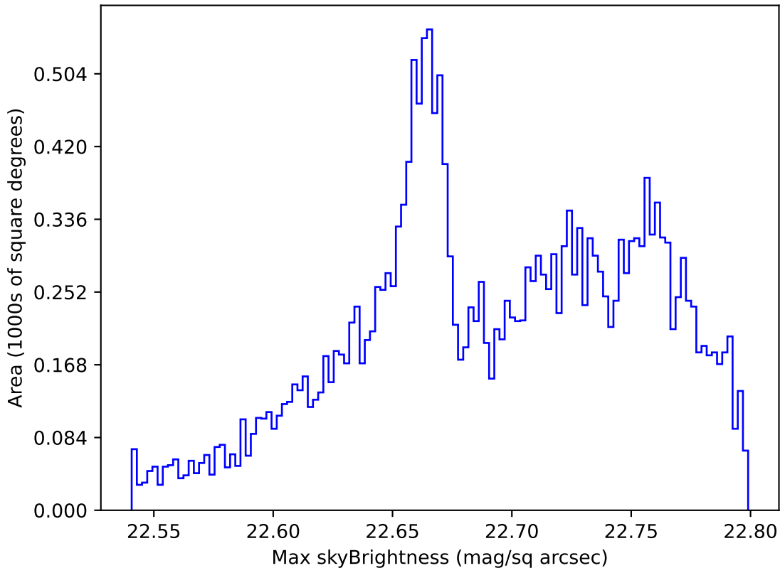
too_elab_r32_d3_griz_v3.4_10yrs All sky u band: Max skyBrightness
