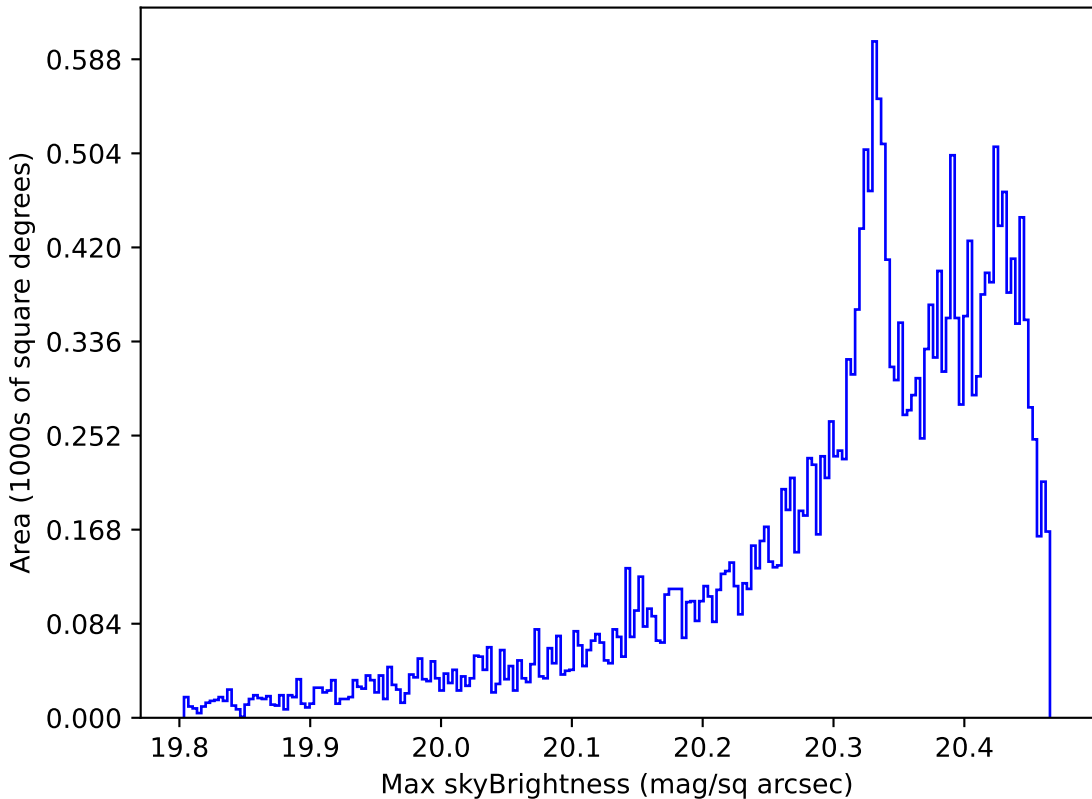
too_elab_r32_d3_griz_v3.4_10yrs All sky i band: Max skyBrightness
