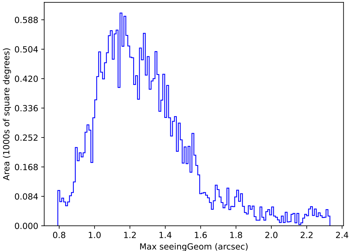
too_elab_r32_d3_griz_v3.4_10yrs Yr 1 z band: Max seeingGeom
