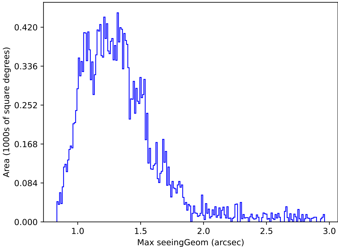
too_elab_r32_d3_griz_v3.4_10yrs Yr 1 u band: Max seeingGeom
