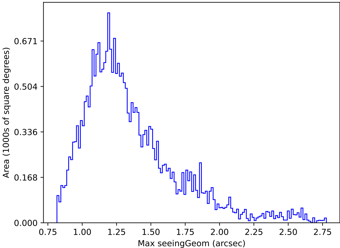
too_elab_r32_d3_griz_v3.4_10yrs Yr 1 i band: Max seeingGeom
