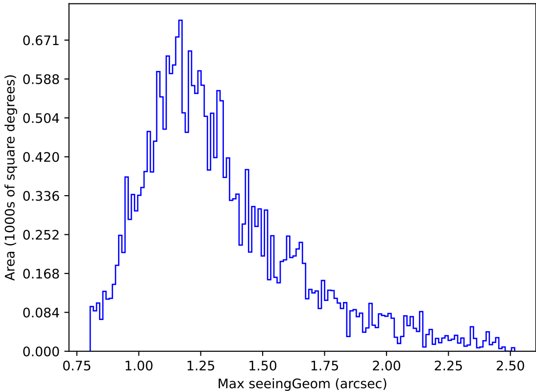
too_elab_r32_d3_griz_v3.4_10yrs Yr 1 g band: Max seeingGeom
