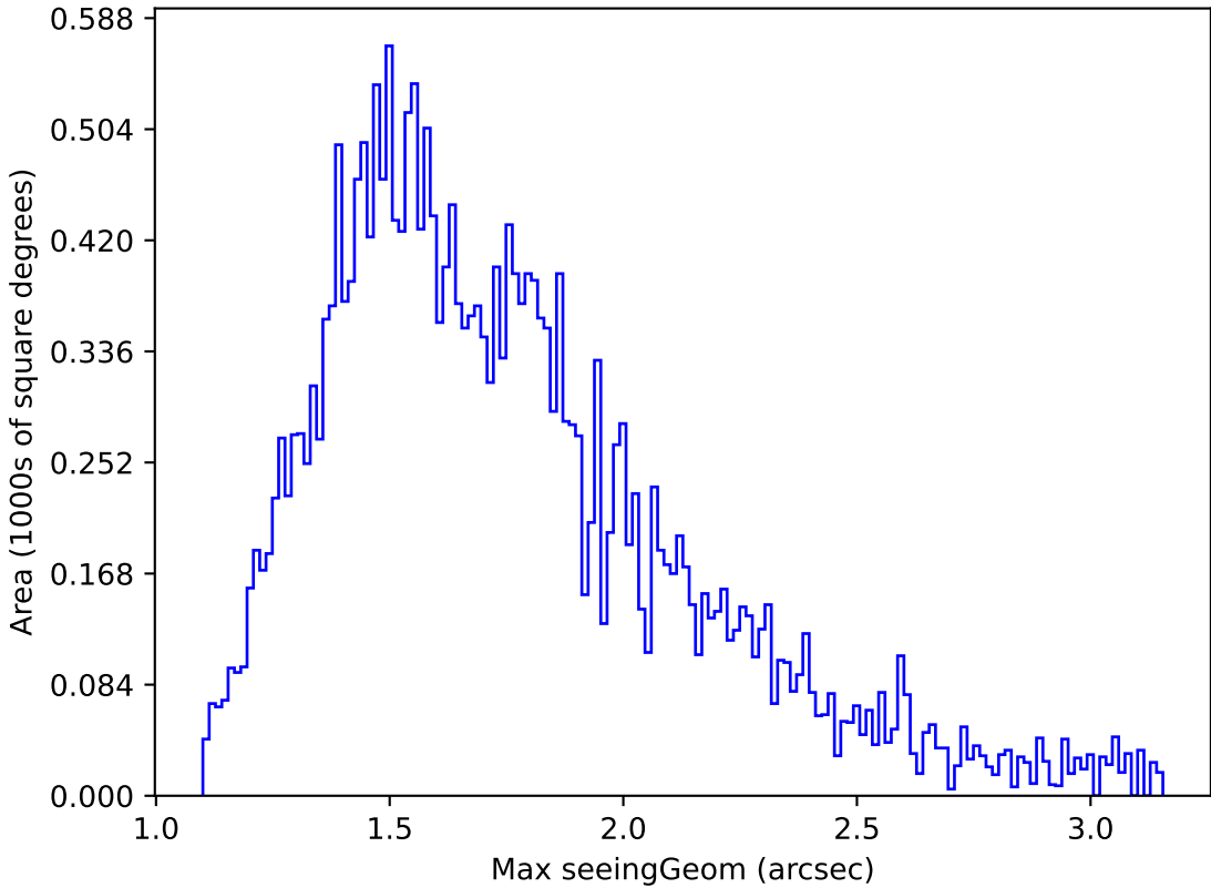
too_elab_r32_d3_griz_v3.4_10yrs Yr 1 all bands: Max seeingGeom
