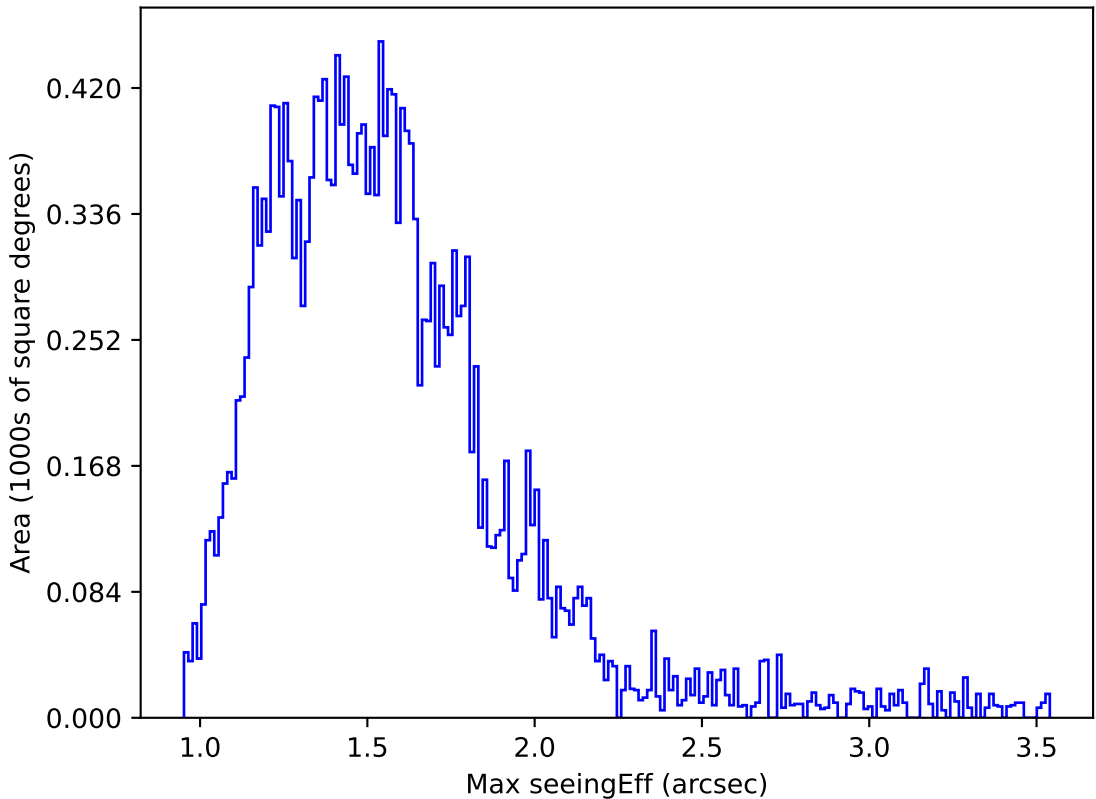
too_elab_r32_d3_griz_v3.4_10yrs Yr 1 u band: Max seeingEff
