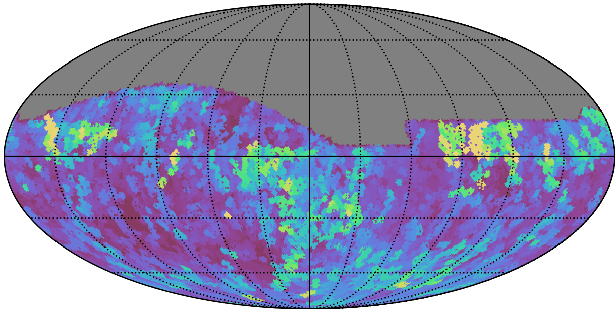
too_elab_r32_d3_griz_v3.4_10yrs Yr 1 all bands: Max seeingEff
