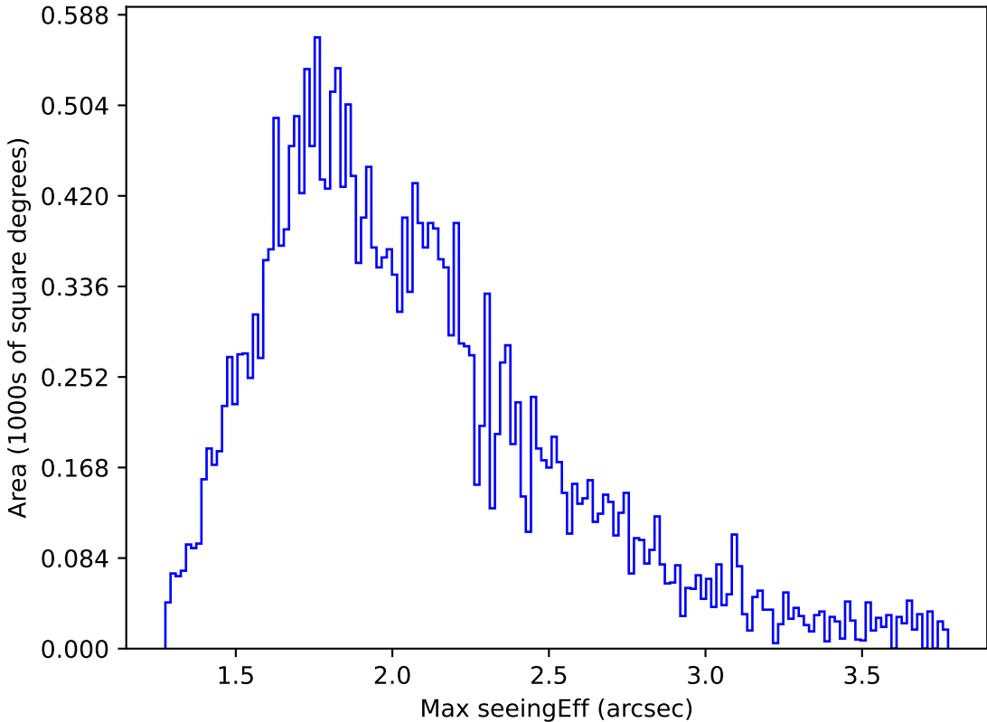
too_elab_r32_d3_griz_v3.4_10yrs Yr 1 all bands: Max seeingEff
