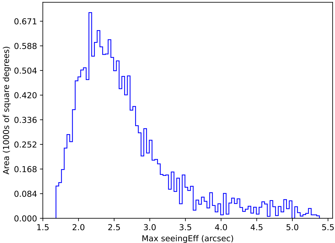
too_elab_r32_d3_griz_v3.4_10yrs WFD z band: Max seeingEff
