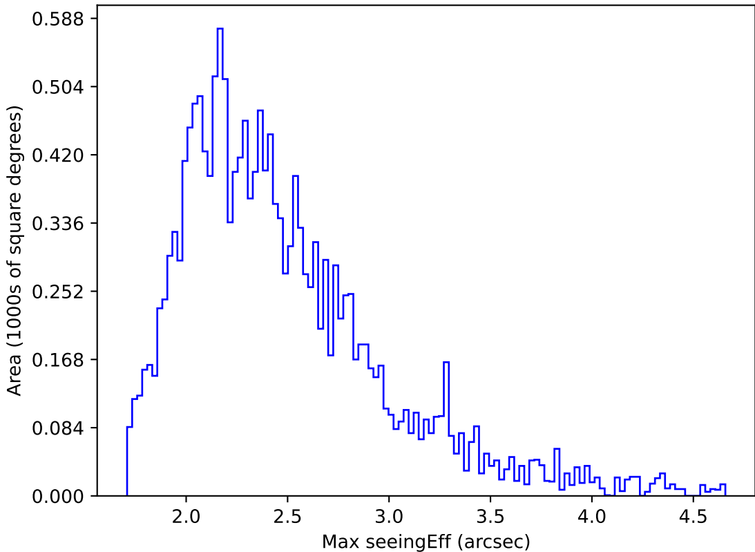
too_elab_r32_d3_griz_v3.4_10yrs WFD u band: Max seeingEff
