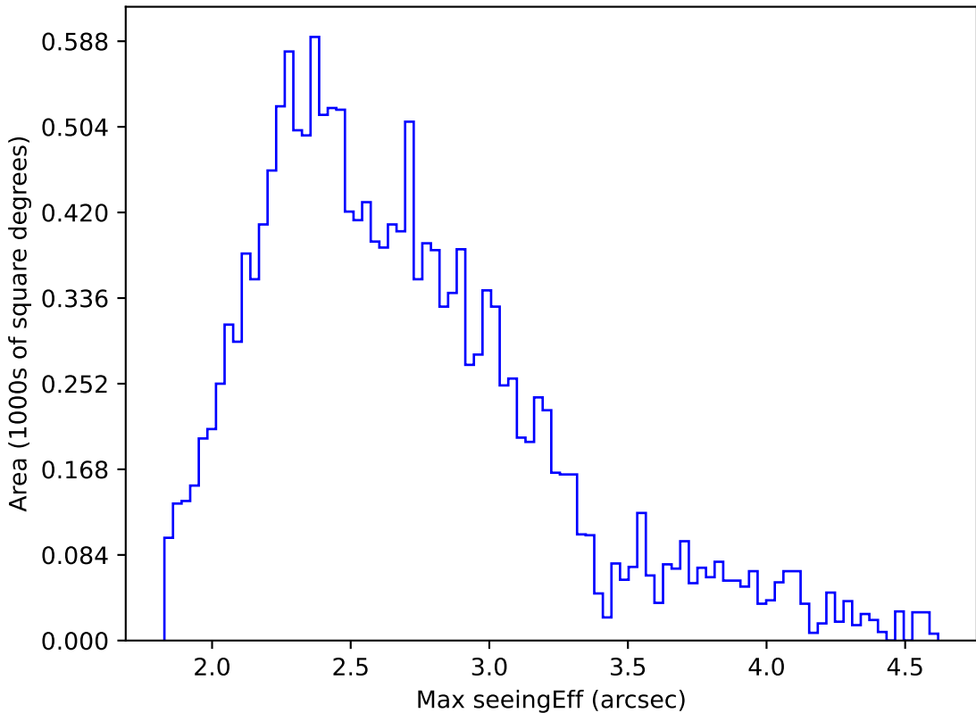
too_elab_r32_d3_griz_v3.4_10yrs WFD r band: Max seeingEff
