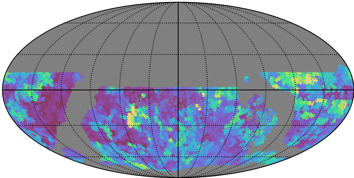
too_elab_r32_d3_griz_v3.4_10yrs WFD g band: Max seeingEff
