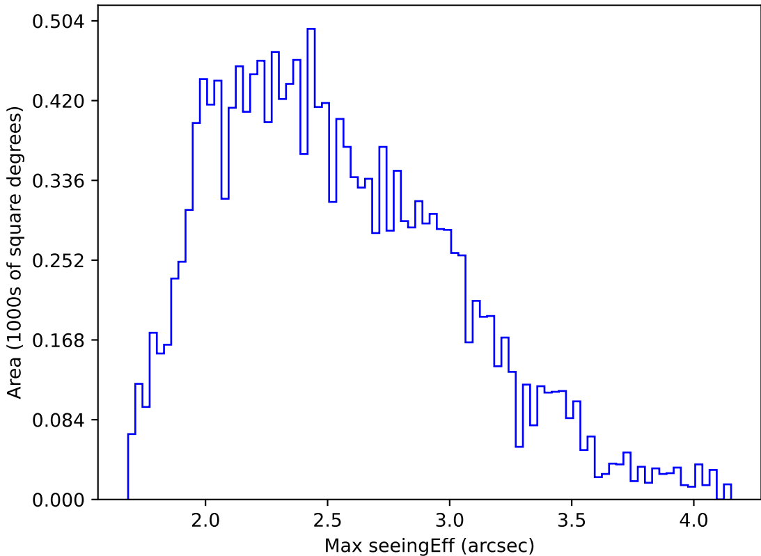
too_elab_r32_d3_griz_v3.4_10yrs WFD g band: Max seeingEff
