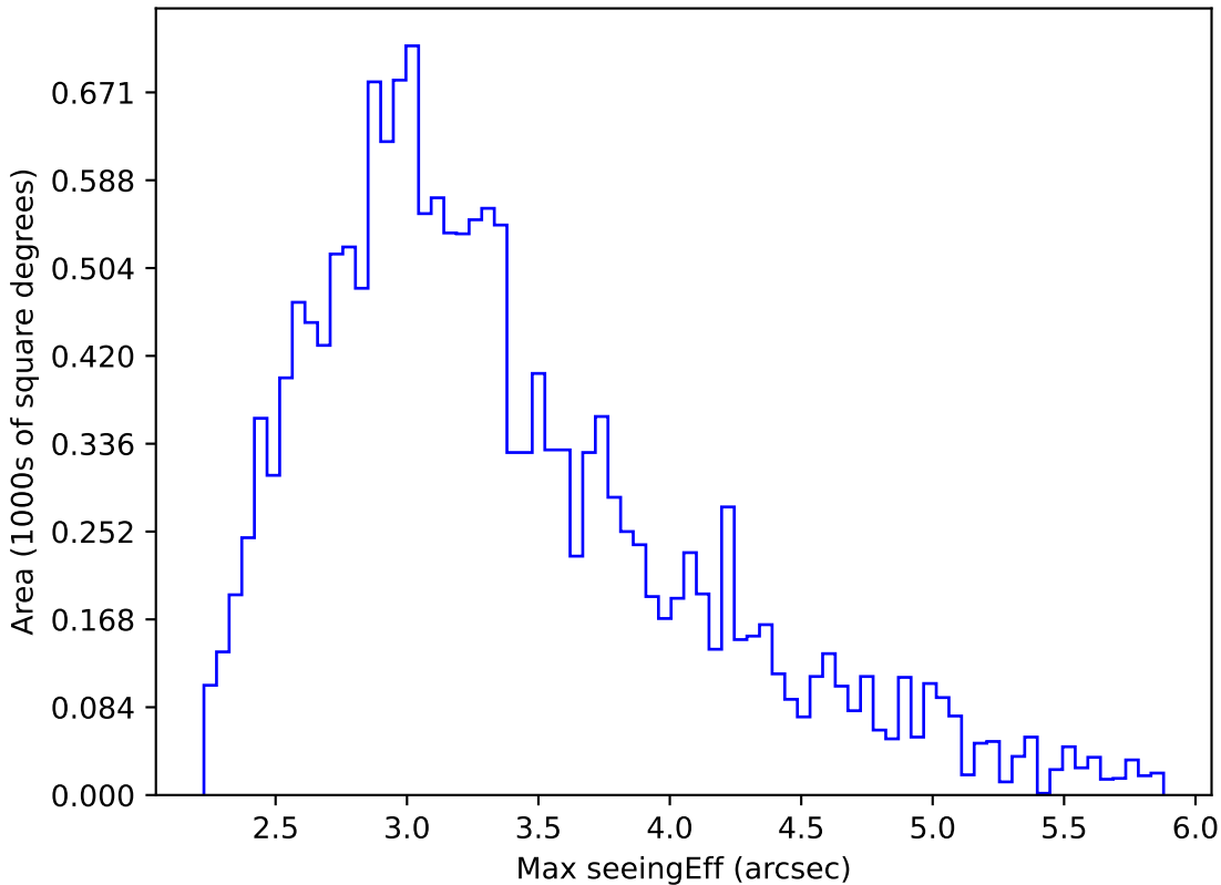
too_elab_r32_d3_griz_v3.4_10yrs WFD all bands: Max seeingEff
