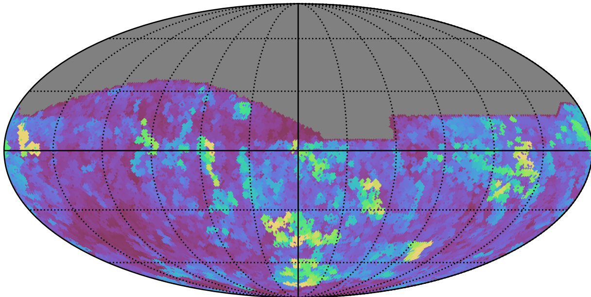
too_elab_r32_d3_griz_v3.4_10yrs All sky z band: Max seeingEff
